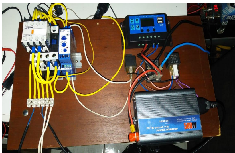
Figura 16: Stringbox
