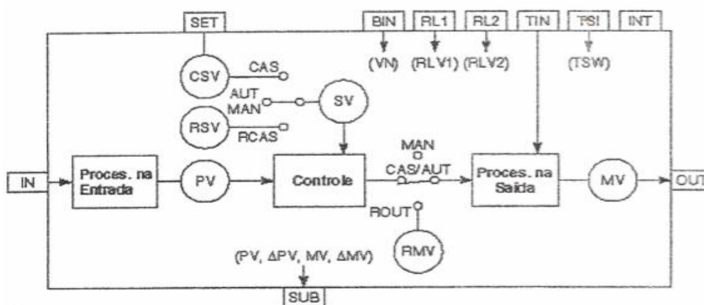
Figura 12: Bloco de Logic chart PID
